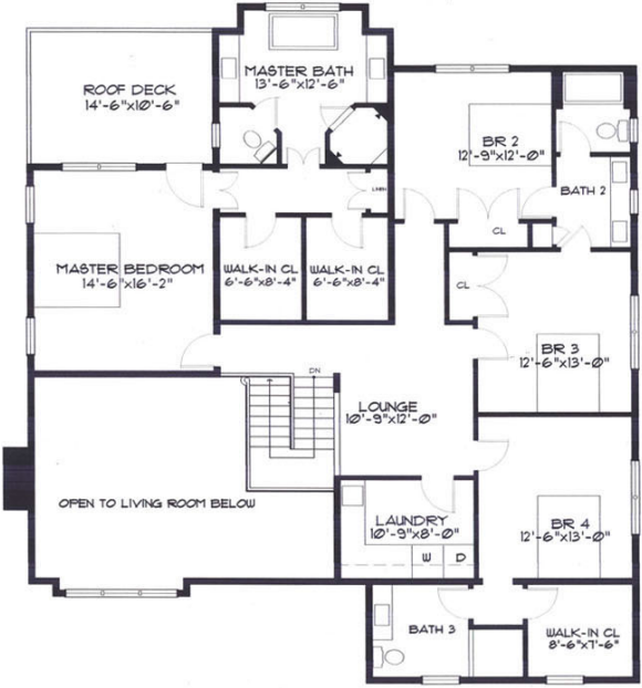
SECOND FLOOR FOUR BEDROOM PLAN
